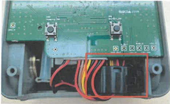
[Main Cable Ferrite Core added]
